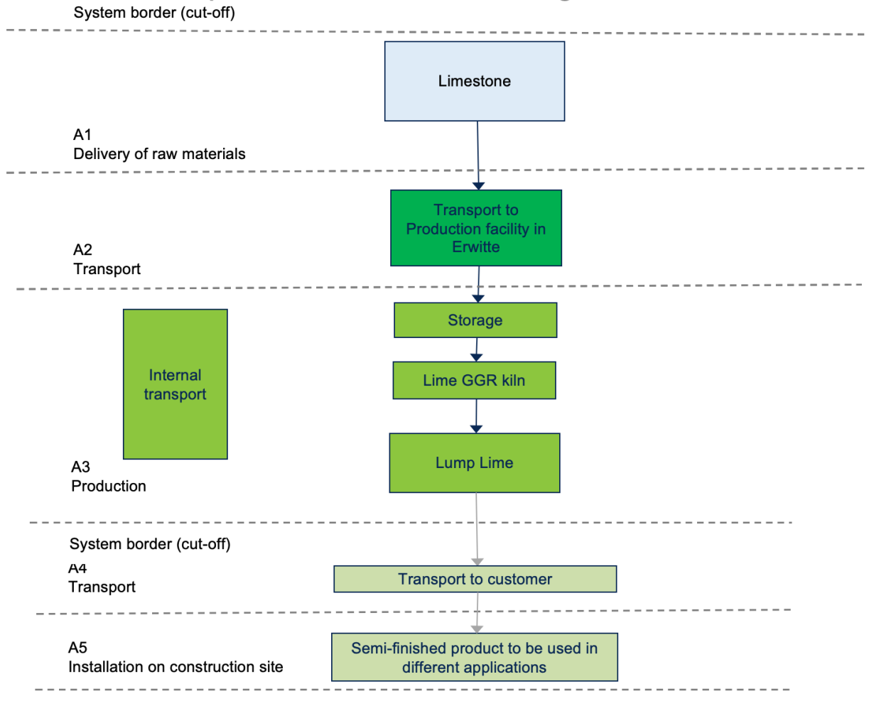
Figure: LCA process diagram according to EN 15804(7.2.1)
